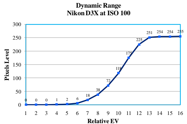
Figure 3. usable dynamic range approximation of 8.5 exposure value with D3X at ISO 100, RAW.
