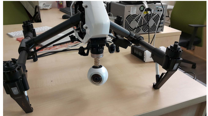
Fig. 2. Retrofitting DJI Inspire with Samsung Gear 360.
